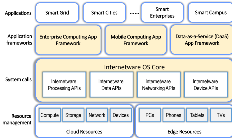
Fig. 3. A prototype architecture for Internetware operating systems. Internetware applications run on top of the cloud and edge devices. The Internetware OS core provides abstractions to manage both cloud and edge resources, while an application framework layer accommodates applications for different domains.
