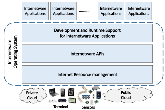
Fig. 2. The concept of an Internetware OS.
