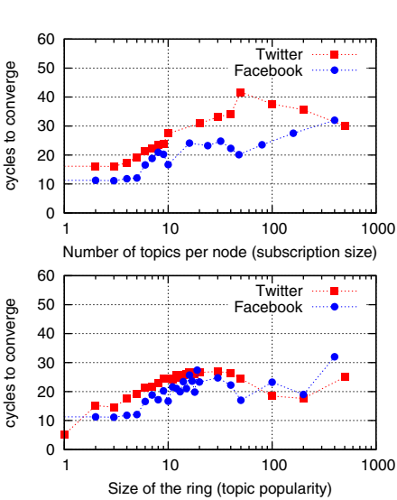
Fig. 6. Correlation between convergence speed and size of the subscription/ring
