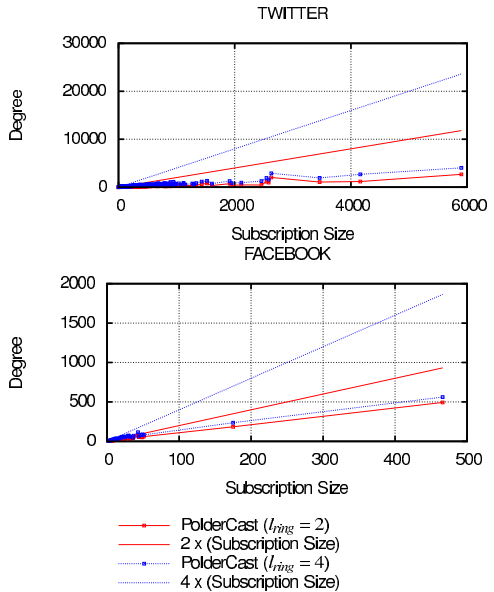
Fig. 7. Node degree in Rings layer
